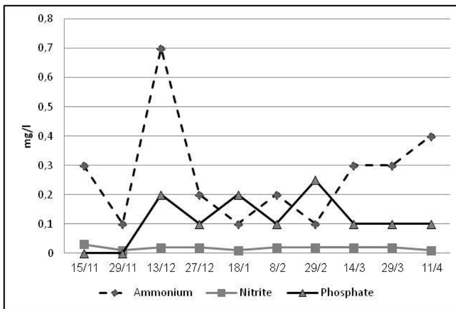
Fig. 2: Variation of nutriments at healthy coastal areas (Oued Maltine)
