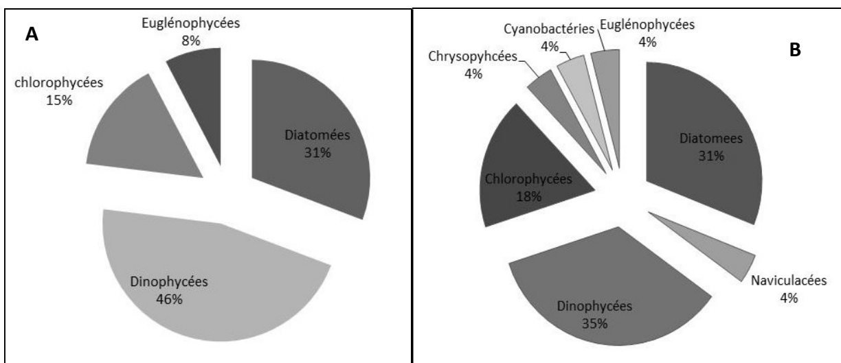
Fig 4: Principals phytoplankton species observed in risky coastal areas (A. Bourgaga lagoon) and healthy coastal areas (B. Oued Maltine)
